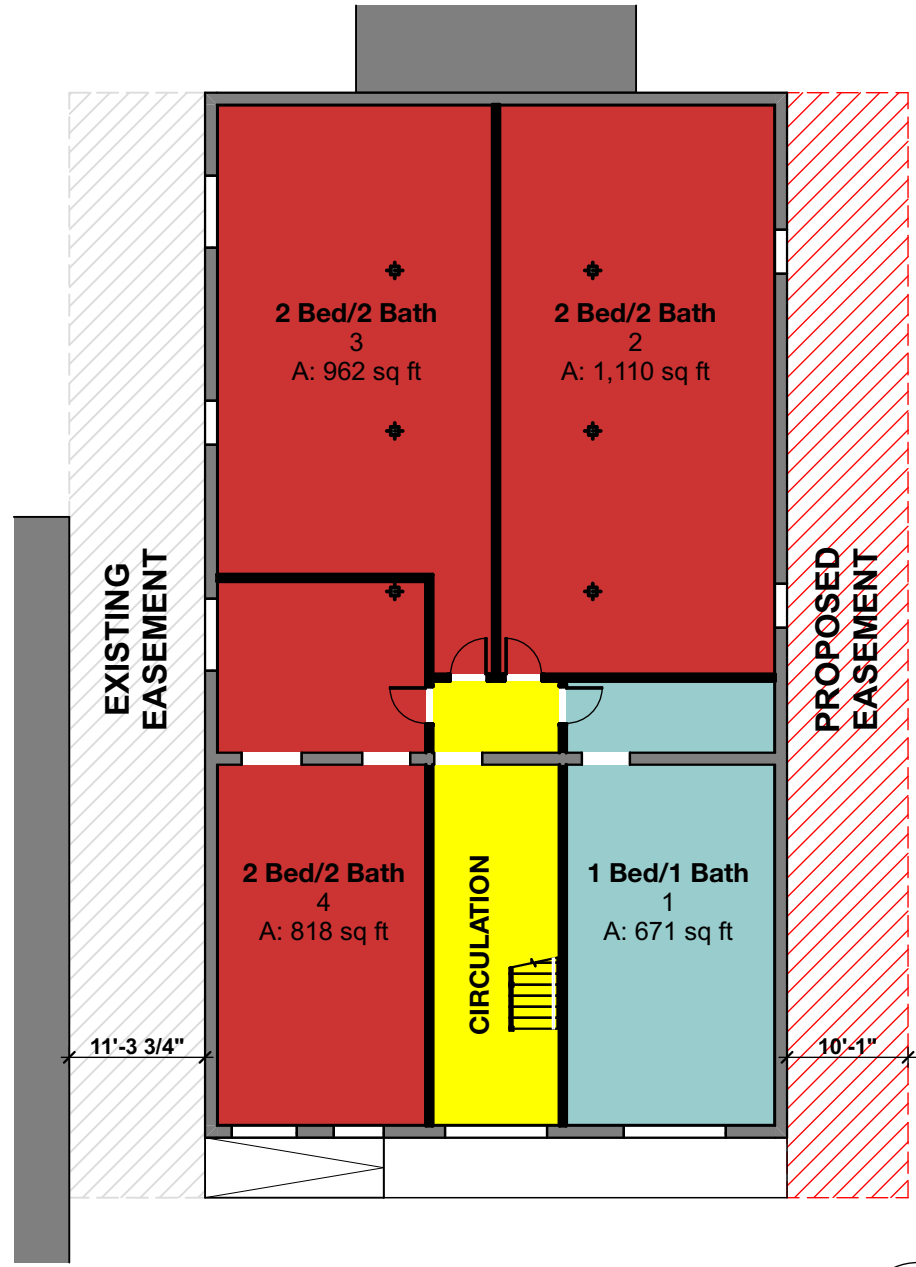
FIRST FLOOR LAYOUT SCALE: 1/16" = 1'-0"
